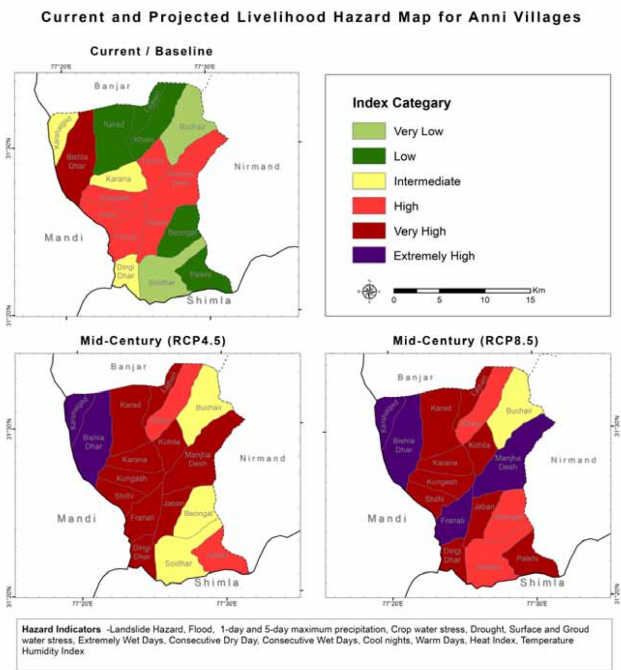
Figure 22: Current and Projected Livelihood Hazard Map for Anni villages, under RCP scenarios 4.5 and 8.5.
