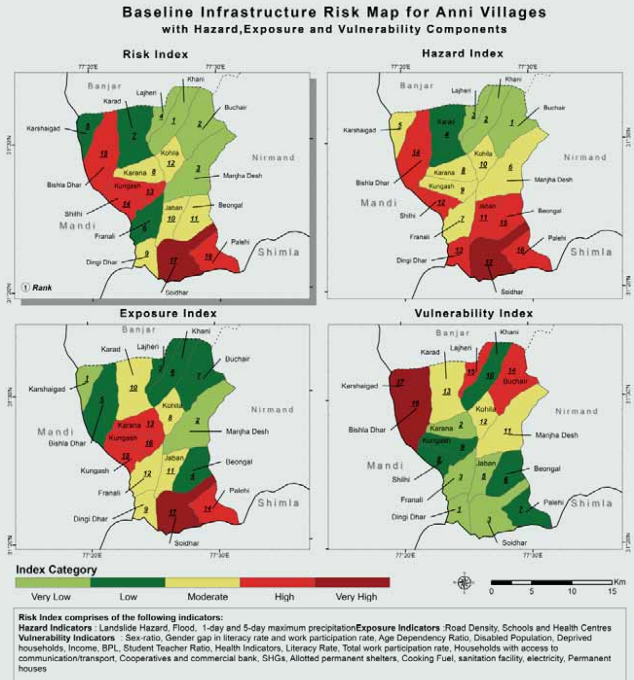
Figure 23: Current Infrastructure Risk Map for Anni villages with Hazard, Exposure and Vulnerability Components
