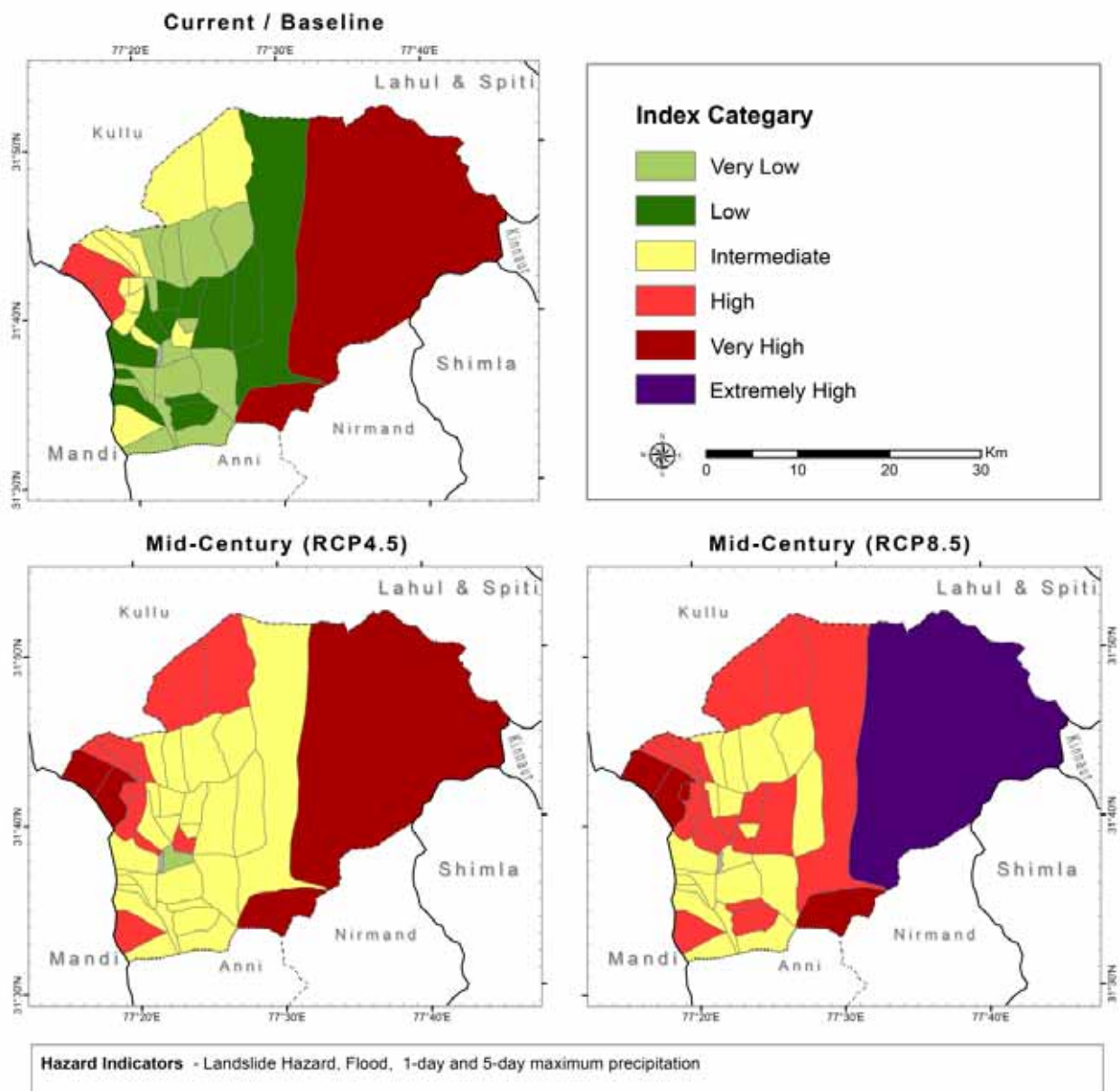
Figure 32: Current and Projected Infrastructure Hazard Map for Banjar villages, under RCP scenarios 4.5 and 8.5.
