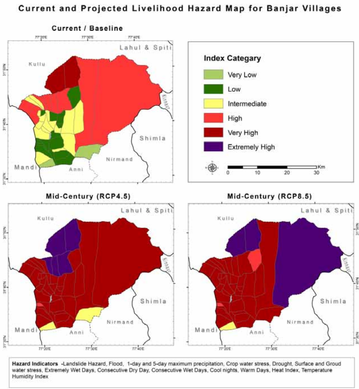
Figure 29: Current and Projected Livelihood Hazard Map for Banjar villages, under RCP scenarios 4.5 and 8.5.
