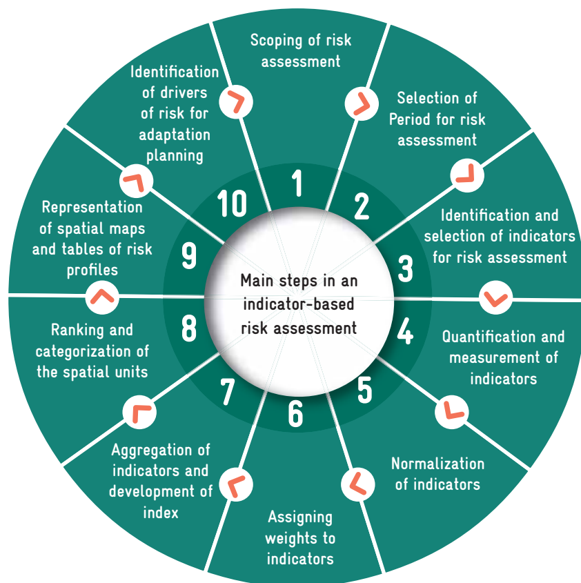
Figure 10: Main steps in an indicator-based risk assessment
