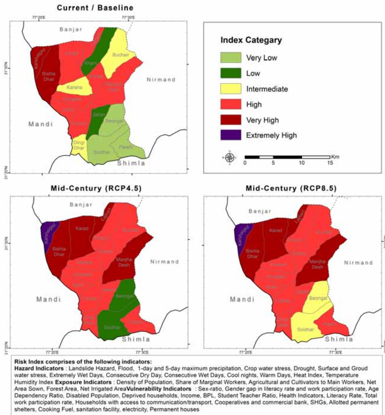
Figure 21: Current and Projected Livelihood Risk Map for Anni villages, under RCP scenarios 4.5 and 8.5.
