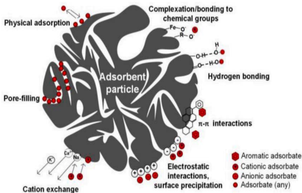
Figure 7.4: Plausible mechanism of pollutant remediation through hydrochar/biochar based adsorbent material.
